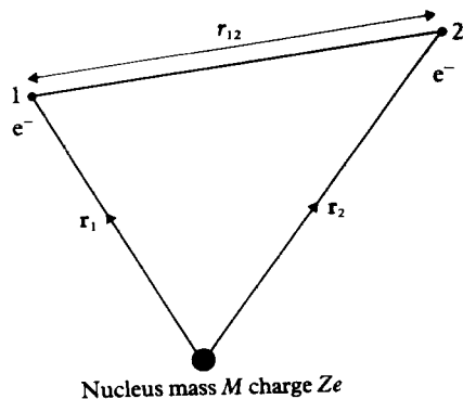
6.1 Coordinate system for two-electron atoms.
